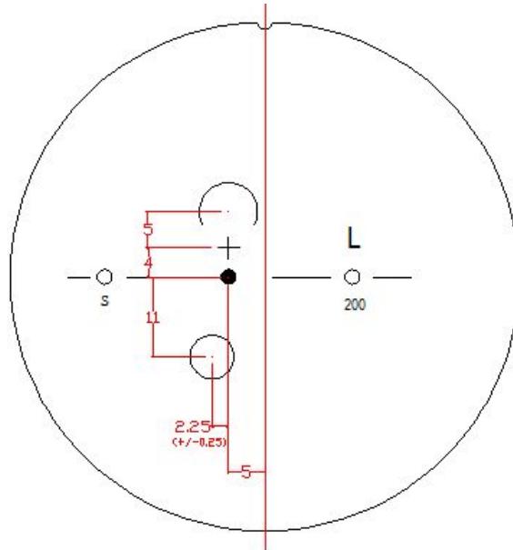
PROGRESSIVE SHORT CORRIDOR (MINIMUM FITTING HEIGHT = 15 MM)
