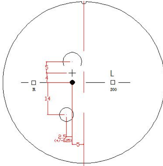
PROGRESSIVE REGULAR CORRIDOR (MINIMUM FITTING HEIGHT = 18 MM)
